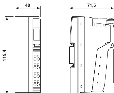
Carcasa BK
